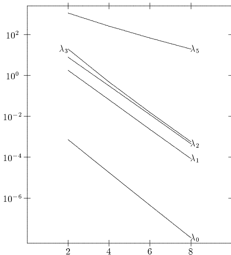
Figure 3. Eigenvalue error: The case of clustered eigenvalues.
