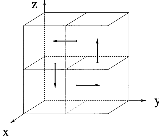
FIG. 2. The curl of a typical potential basis function
