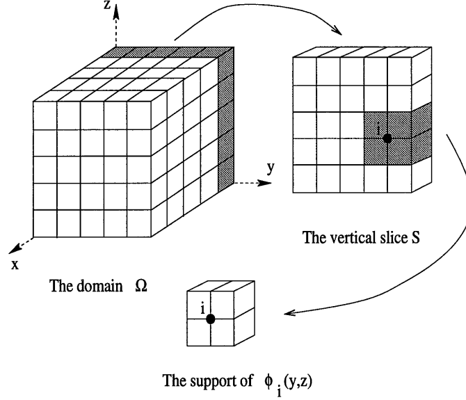
FIG. 1. The support of a typical potential basis function
