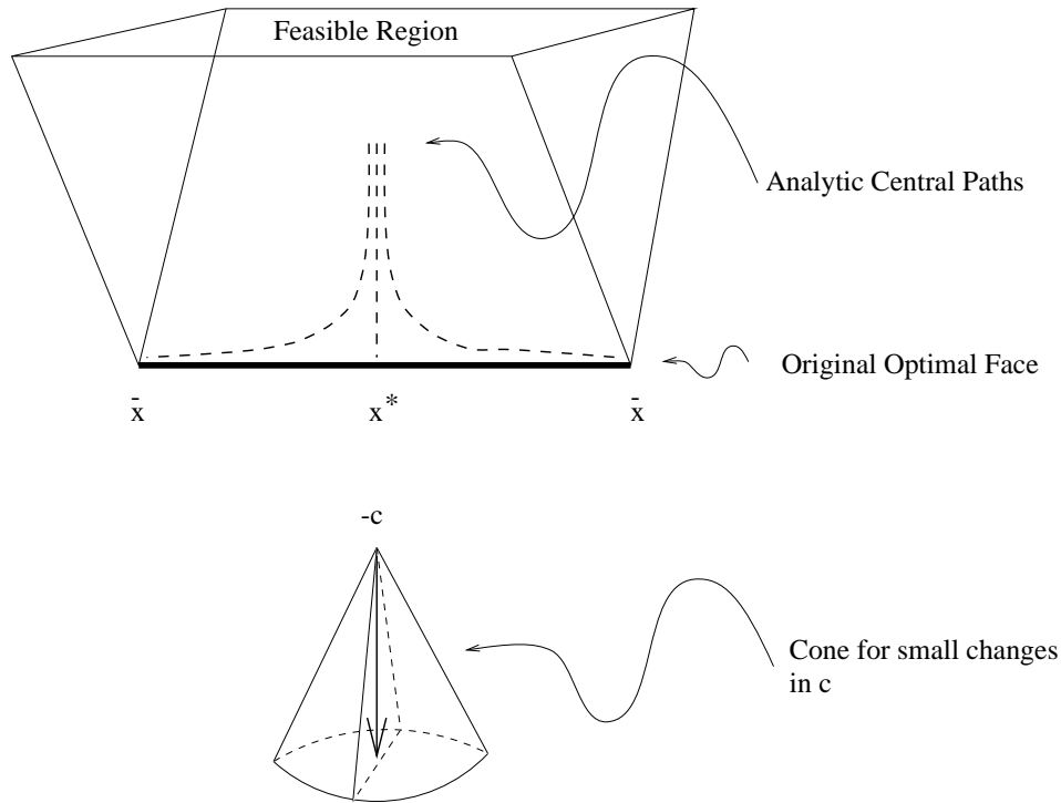
Figure 1: The vector in the center of the cone is -c . If the perturbed vector lies in the cut through the cone, then the central optimal solution remains intact. Hence, \delta c \in \mathcal{H}_c^1 . Otherwise, the new central optimal solution is located at one of the \bar{x} 's, and \delta c \in \mathcal{H}_c \setminus \mathcal{H}_c^1 .
