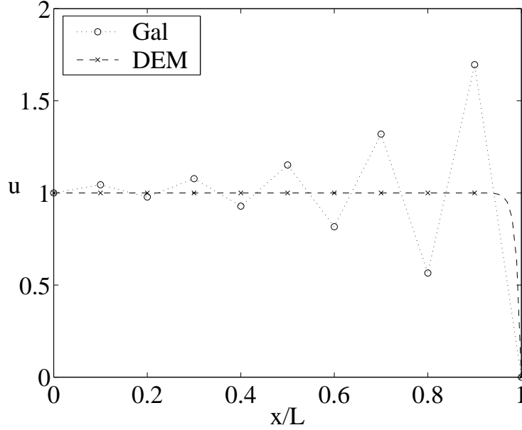
Fig. 23. Homogeneous problem in one dimension, \alpha = 5 .
